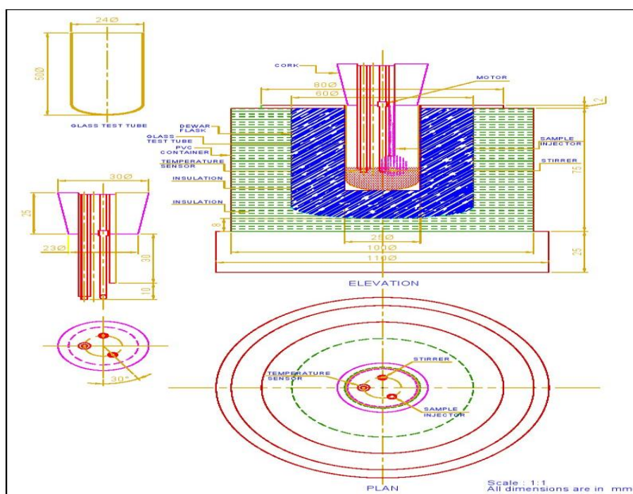
Fig 1 Calorimeter Design
