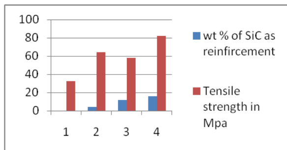
Tensile strength of sic Reinforcement
