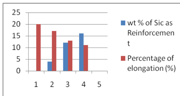
Percentage of Elongation of specimens
