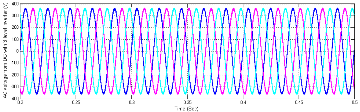
Figure 7: AC voltage from DG with 3-level inverter
