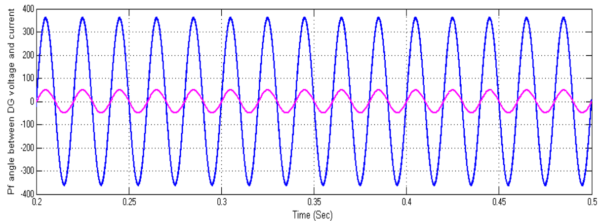
Figure 26: Power factor angle between DG voltage and current
