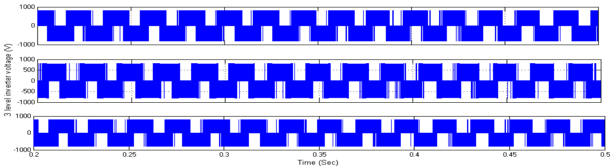
Figure 9: 3-level inverter output voltage
