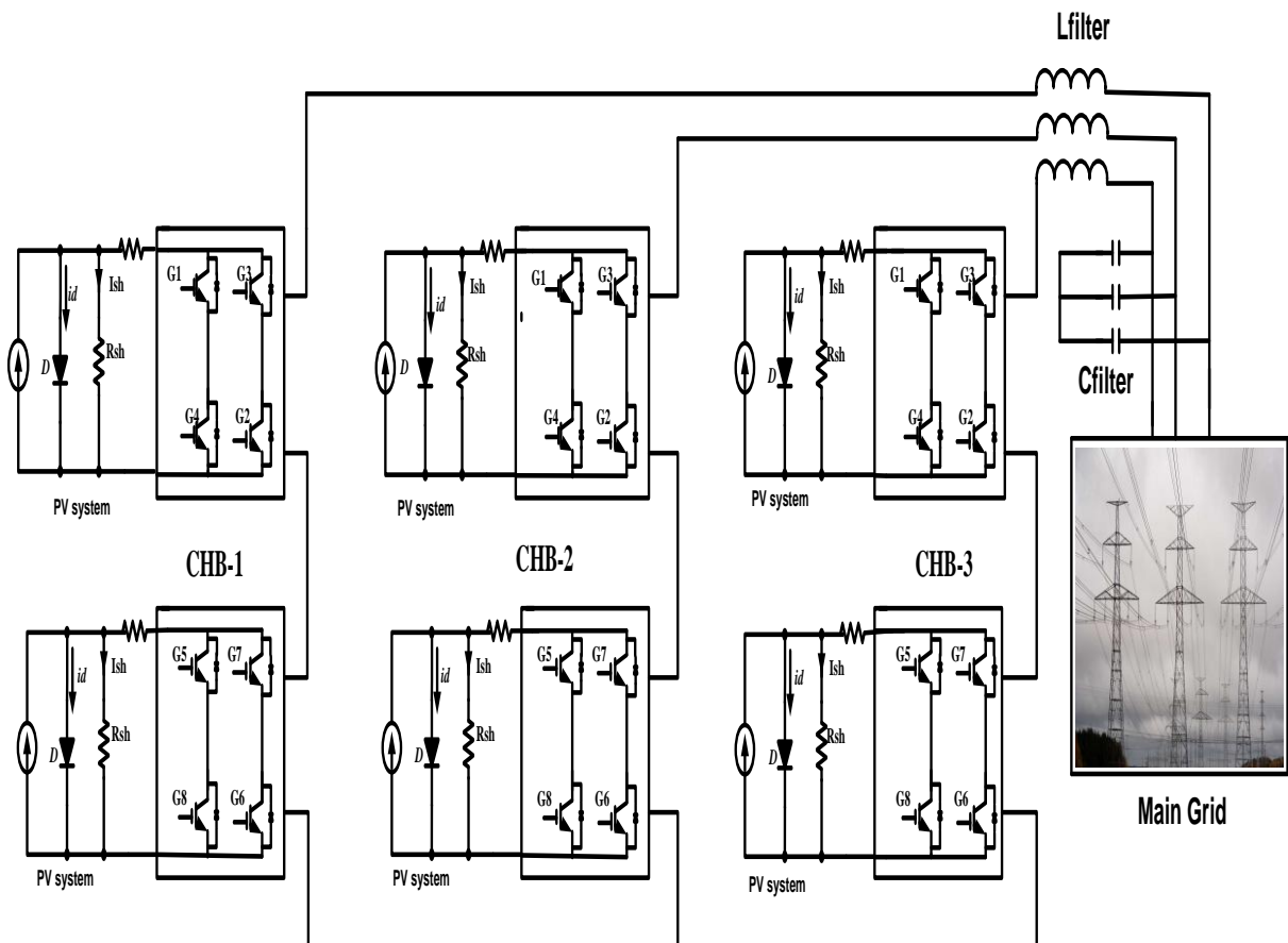
Figure 4: PV system integration to grid with three-phase CHB inverter
