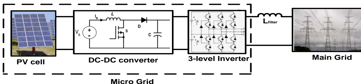
Figure 1: Typical PV based system integration to main grid
