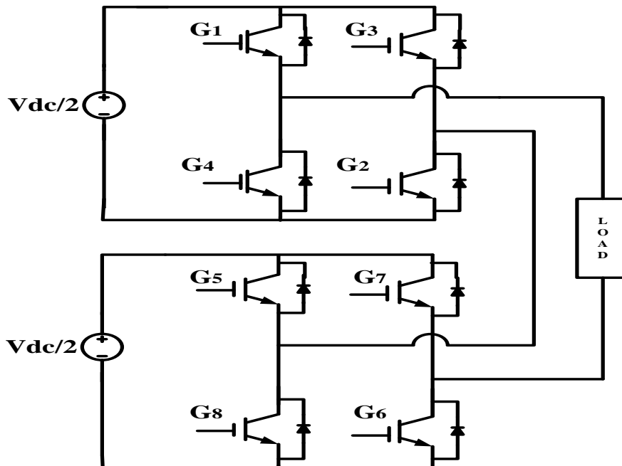
Figure 3: 5-level CHB inverter topology per phase
