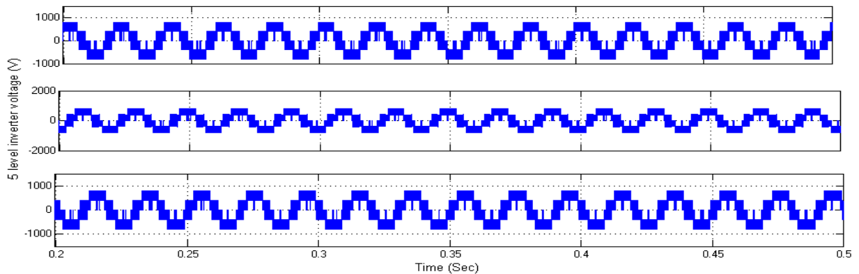
Figure 23: 5-level inverter output voltage
