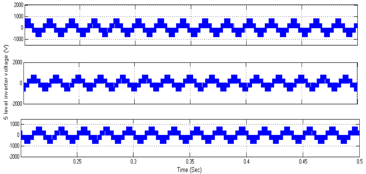
Figure 30: 5-level inverter output voltage
