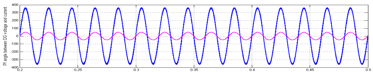
Figure 12: Power factor angle between DG voltage and current
