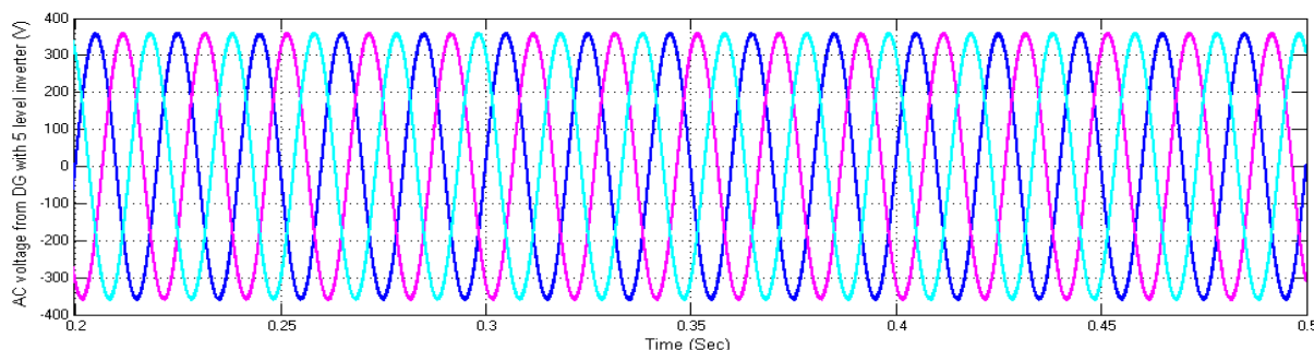
Figure 28: AC voltage from DG with 5-level inverter
