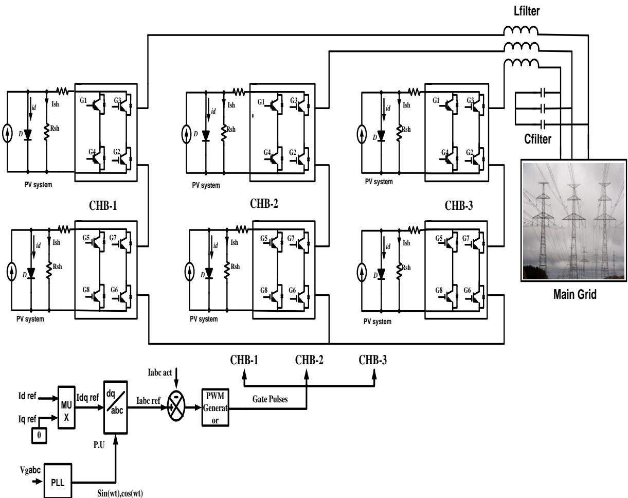
Figure 6: Complete schematic arrangement of PV integration to grid through multi-level inverter with control block
