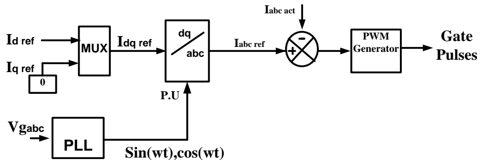
Figure 5: Control block diagram for inverters
