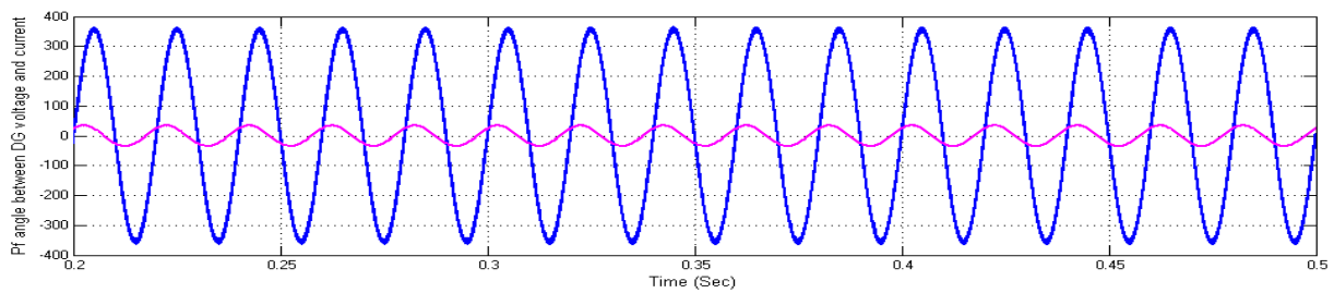
Figure 19: Power factor angle between DG voltage and current
