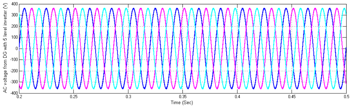
Figure 21: AC voltage from DG with 5-level inverter
