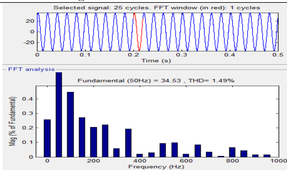
Figure 33: THD of DG current with 5 level inverter
