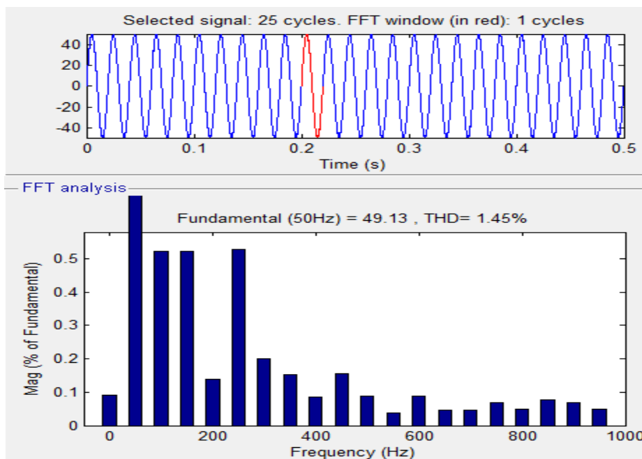
Figure 27: THD of DG current in 5 level inverter
