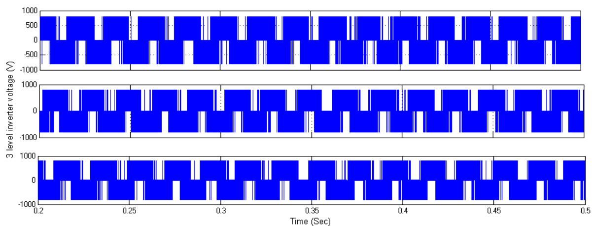
Figure 16: 3 level inverter voltage
