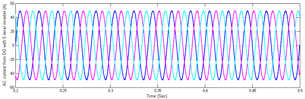
Figure 22: AC current from DG with 5-level inverter
