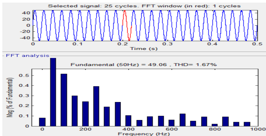
Figure 13: THD of DG current with 3 level inverter
