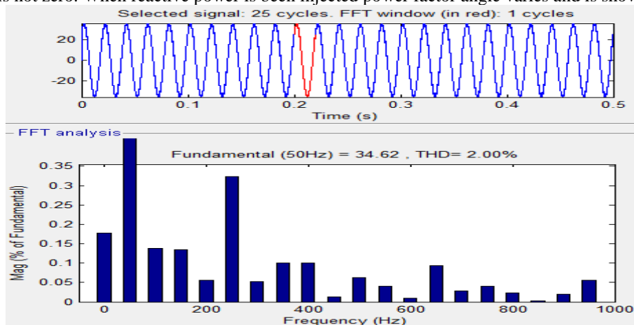
Figure 20: THD of DG current with 3 level inverter
