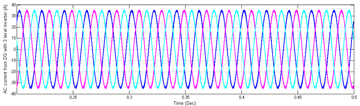
Figure 15: AC current from DG with 3 level inverter
