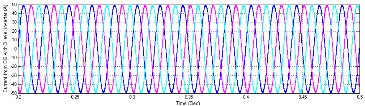
Figure 8: AC current from DG with 3-level inverter
