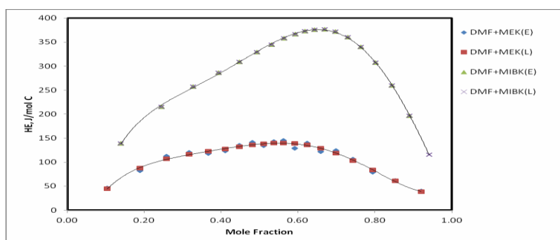
Fig.3: DMF with ketones
