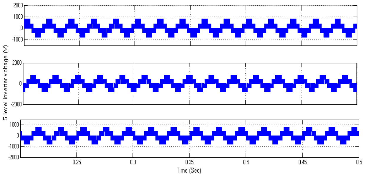
Figure 30: 5-level inverter output voltage
