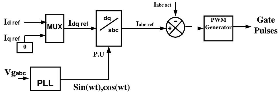
Figure 5: Control block diagram for inverters
