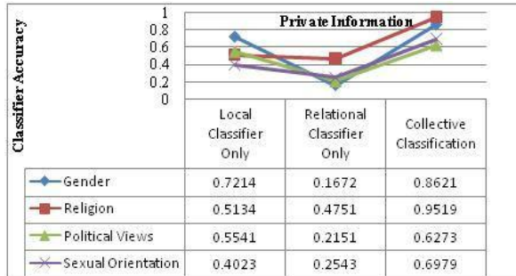
Fig.5.1 Calculating Classifier Accuracy
