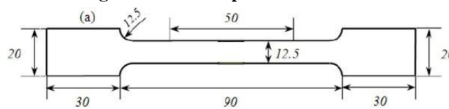
Fig 3. Tensile test specimen dimension
