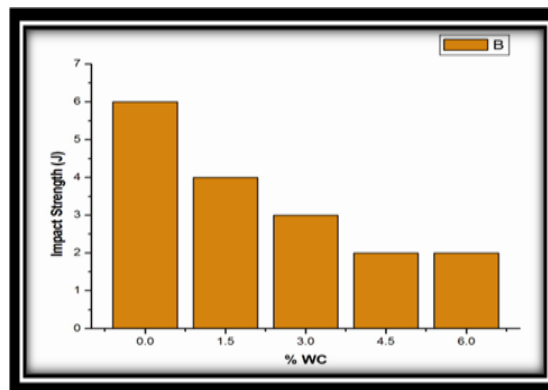
Fig 6: The effects of percentage of WC particulates on the toughness of MMCs
