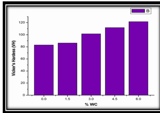
Fig 5: the effects of percentage of WC particles on the hardness of MMCs
