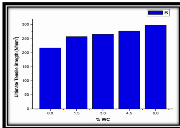
Fig 4: the effects of percentage of WC particles on the Ultimate Tensile Strength of MMCs
