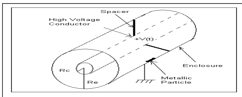
I. Schematic diagram of a typical GIB
