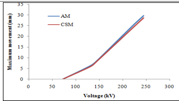
Fig 6. Maximum movement of copper particles( l=20\text{mm} , r=0.25\text{mm} ) at different voltages
