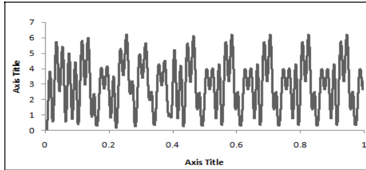
Fig 3.MOVEMENT OF ALUMINIUM PARTICLE (L=20MM, R=0.25MM) AT 72.5 kV USING ANALYTICAL FIELD
