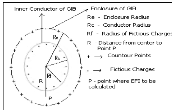
Fig 2. Basic Concept of Charge Simulation Method
