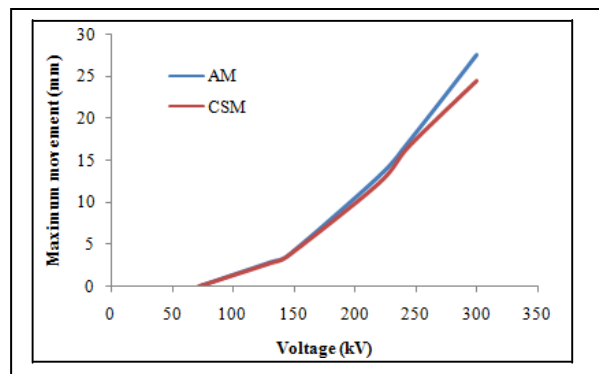
Fig .8 Maximum movement of copper particles( r=0.25\text{mm} ) of different lengths
