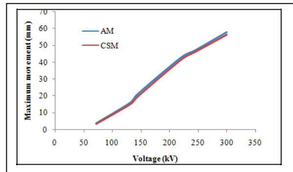
Fig .9 Maximum movement of copper particles ( l=10\text{mm} ) of different radii
