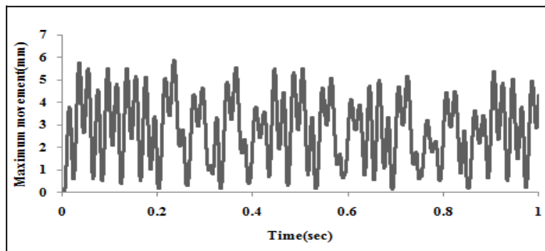
Fig 4. Movement of aluminium particle (l=20mm, r=0.25mm) at 72.5 kV using Charge simulation method
