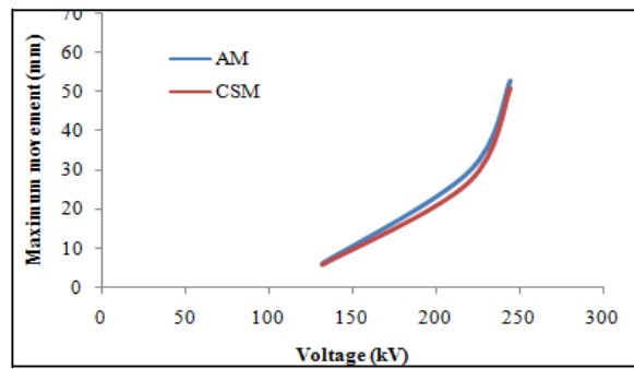
Fig .7 Maximum movement of aluminium particles( l=20\text{mm} , r=0.25\text{mm} ) at different voltages
