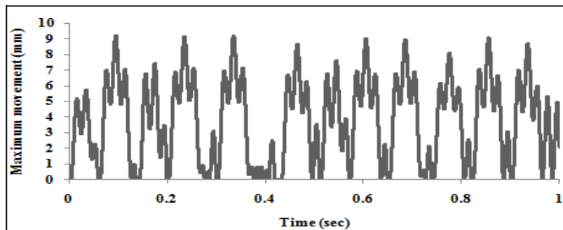
Fig 5.Movement of copper particle (l=15mm, r=0.35mm) at 220 kV using Analytical method
