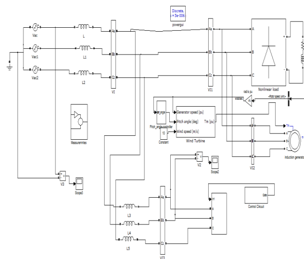
Figure 6: Simulation Diagram of proposed system with TSC
