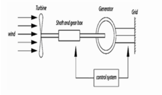
Figure 2 Basic schematic diagram of wind turbine
