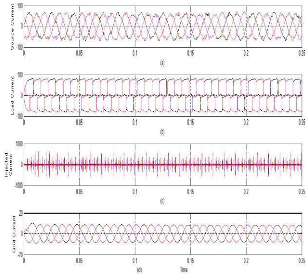
Figure 7: Results for Wind Energy System with TSC
