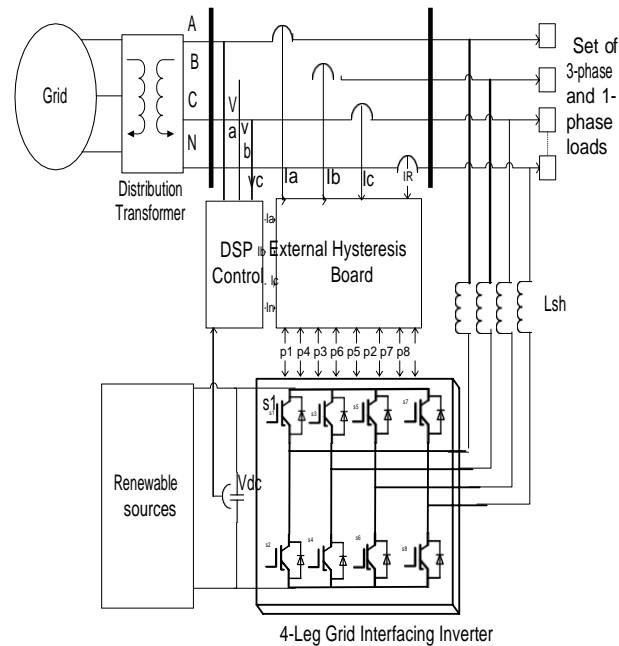
Figure 1: Diagram for Proposed System.
