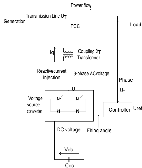
Figure 4: Basic block diagram for static compensator.
