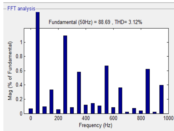
Fig 11: FFT analysis for Source current.
