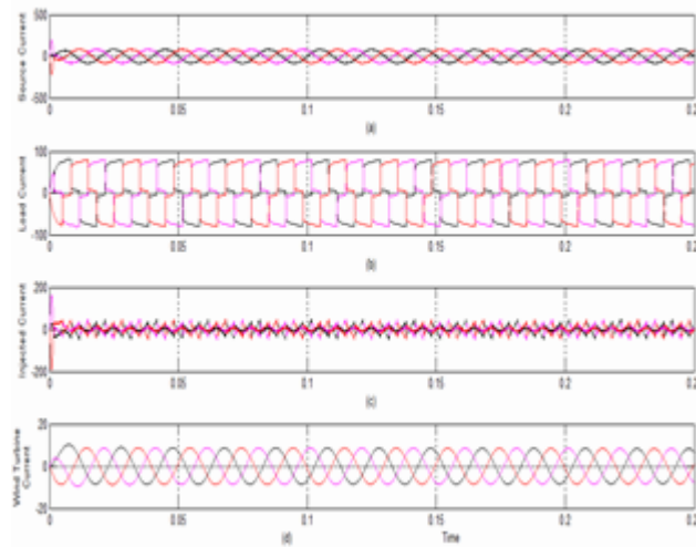
Figure 10: simulation result for current.
