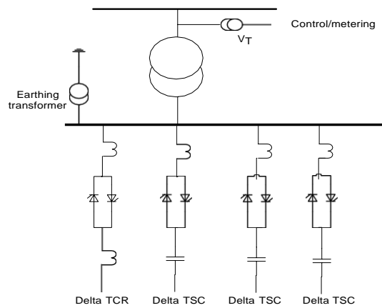
Figure 5: Thyristor Switched Capacitor
