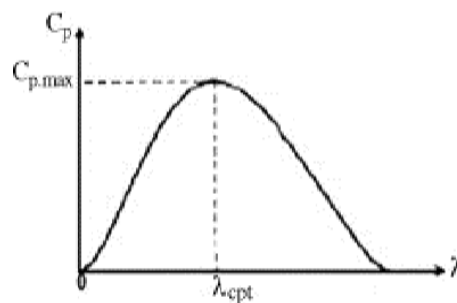
Figure 3: Power coefficient Vs Tip Speed Ratio
