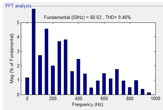
Figure 8: FFT analysis for Source current.
