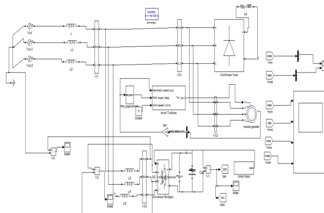
Figure 9: Over All Circuit Diagram in Simulation with Sub Systems
