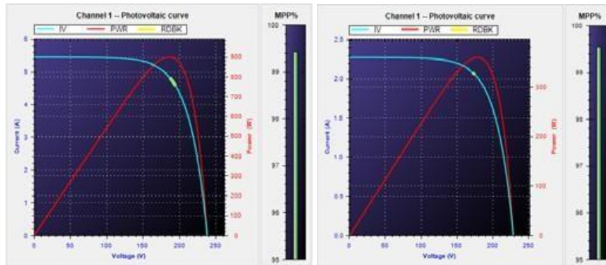
Fig. 7 MPPT performance at (a) 1000 W/m 2 , (b) 400 W/m 2
