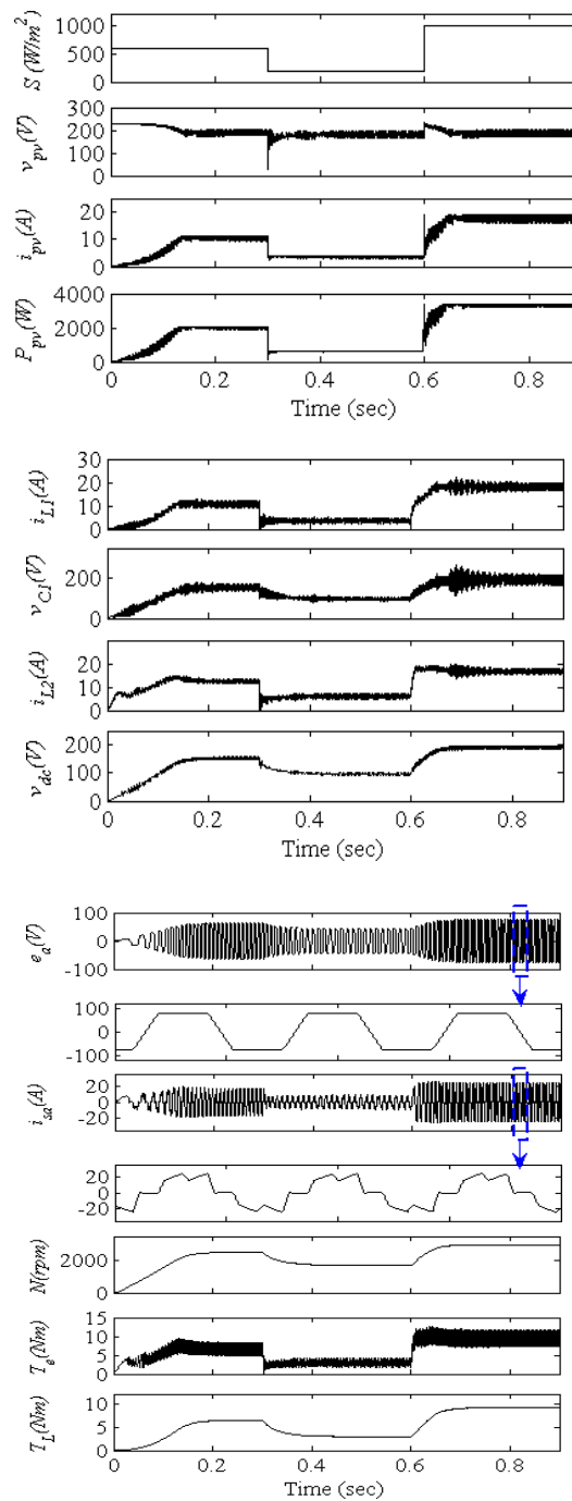
Fig. 5 Dynamic performances of the proposed SPV array based Zeta converter fed BLDC motor drive for water pump (a) SPV array variables, (b) Zeta converter variables, and (c) BLDC motor-pump variables.
