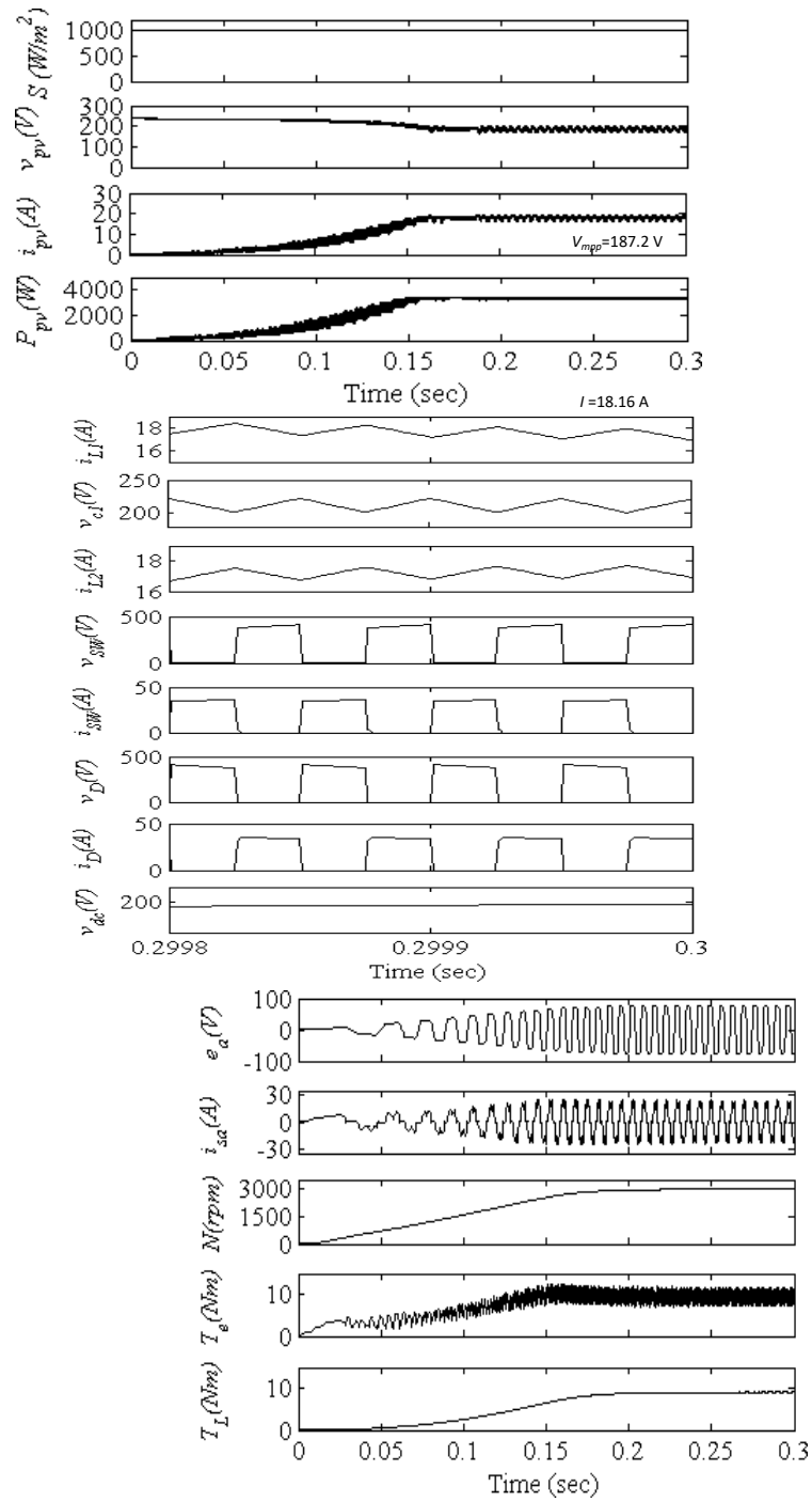
Fig. 4 Starting and steady state performances of the proposed SPV array based Zeta converter fed BLDC motor drive for water pump (a) SPV array variables, (b) Zeta converter variables, and (c) BLDC motor-pump variables.
