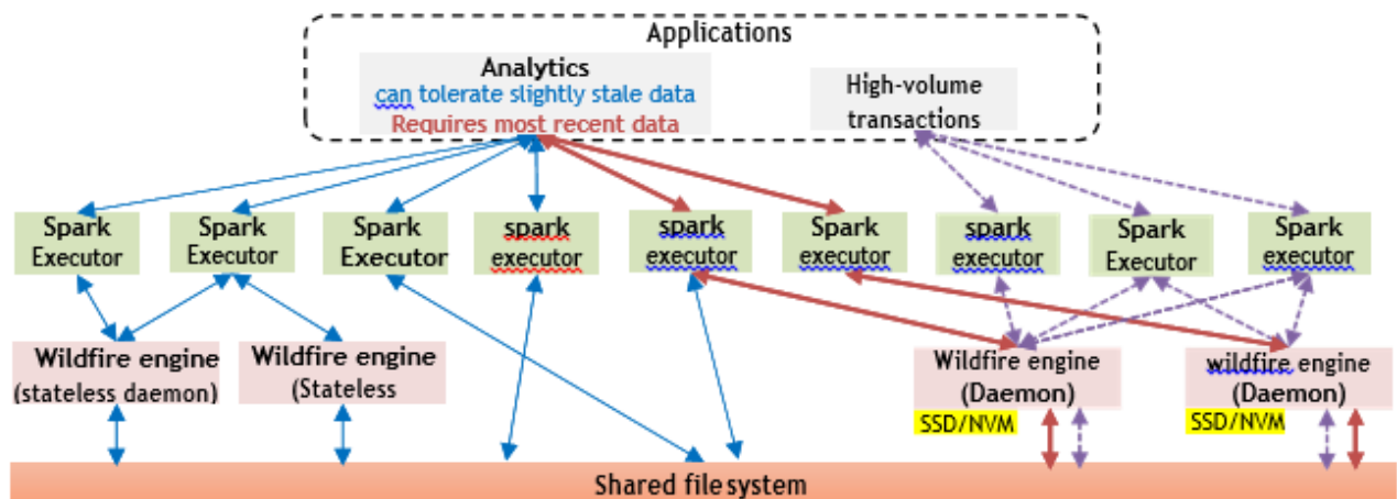
Figure 1: Wildfire Architecture.
