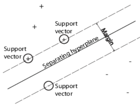
Fig 6. SVM Algorithm
