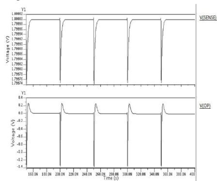
Figure 5 . Output of Vddt sensor implementation
