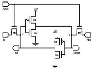
Figure 1: 6T CMOS SRAM cell
