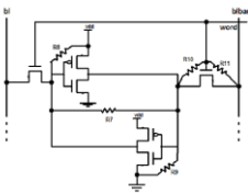
Figure 3: Bridging faults in SRAM
