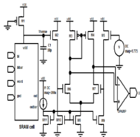
Figure 4: VDDT Sensor
