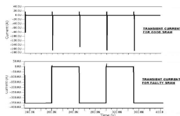
Figure 6 . Difference in transient current
