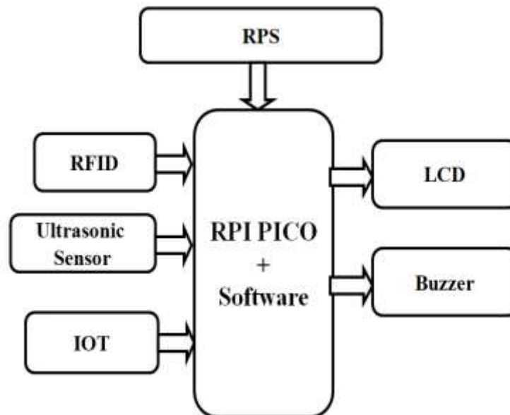
Fig.1. Block diagram
