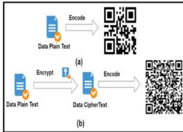
4.1. System Architecture
