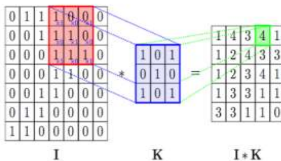
Fig 2. Convolutional layer
