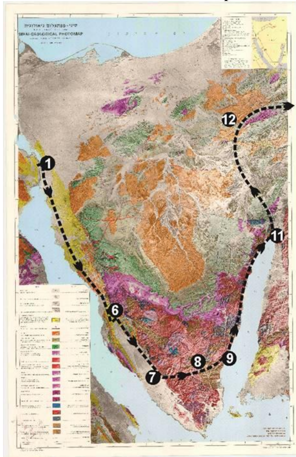
Figure 2. : Sinai – Geological Photomap, Eyal., et., all 1980
