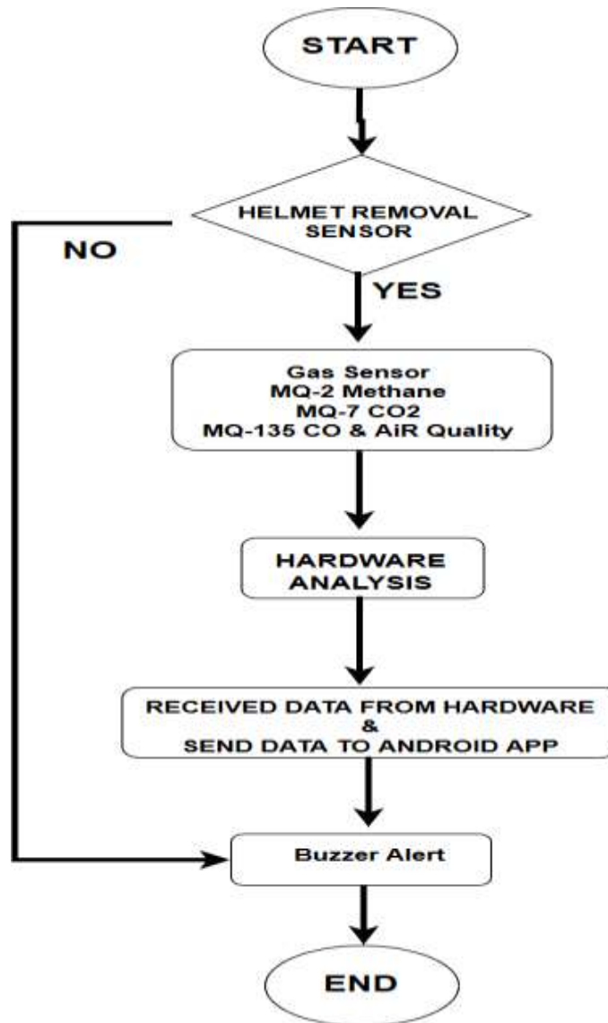
FIGURE 3.5: Mine Gas Monitoring Dangerous level.
