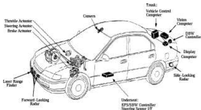
Fig. 8. OSU Autonomous Vehicle [21]
