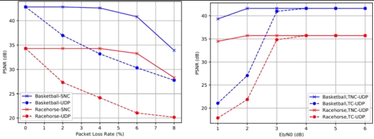
Fig. 3 PSNR for SNC and UDP protocol at packet loss rates of 2,4, 6, and 8% for the two video sequences at 1Mbps.
