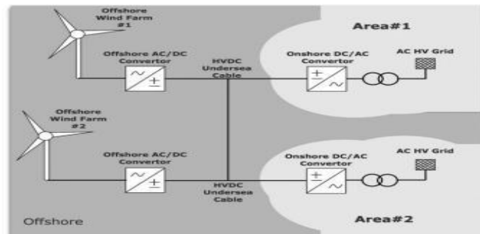
Figure.6. MTDC grid test system.
