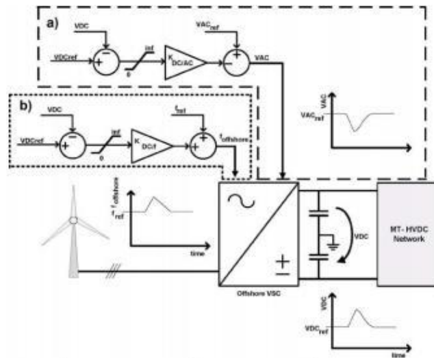
Figure 5. Control scheme for FRT provision based on dc voltage: (a) AC offshore grid voltage control. (b) AC offshore grid frequency control.
