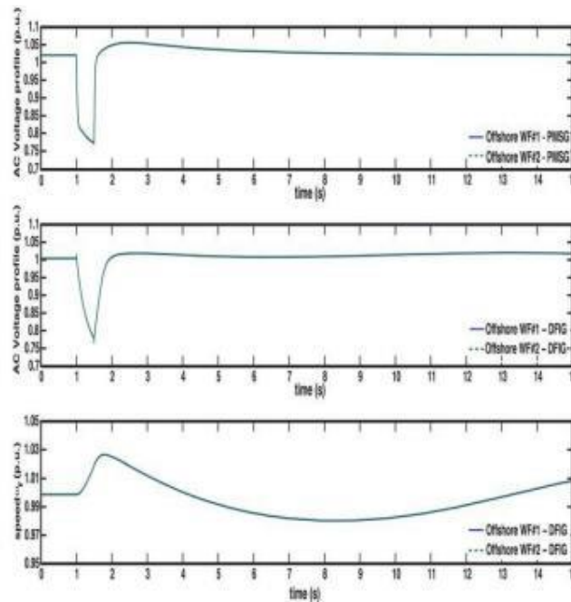
Figure10. AC voltage profile at offshore network and DFIG speed.
