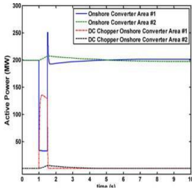
Figure 9. Onshore converter and dc choppers active power Onshore Chopper Resistors
